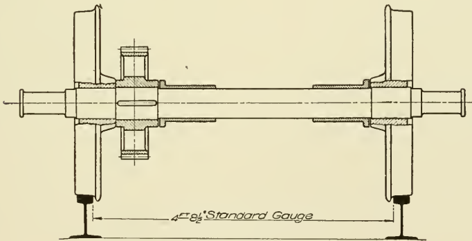
Fig. 26. Part Section of Wheels, Axle and Gear
